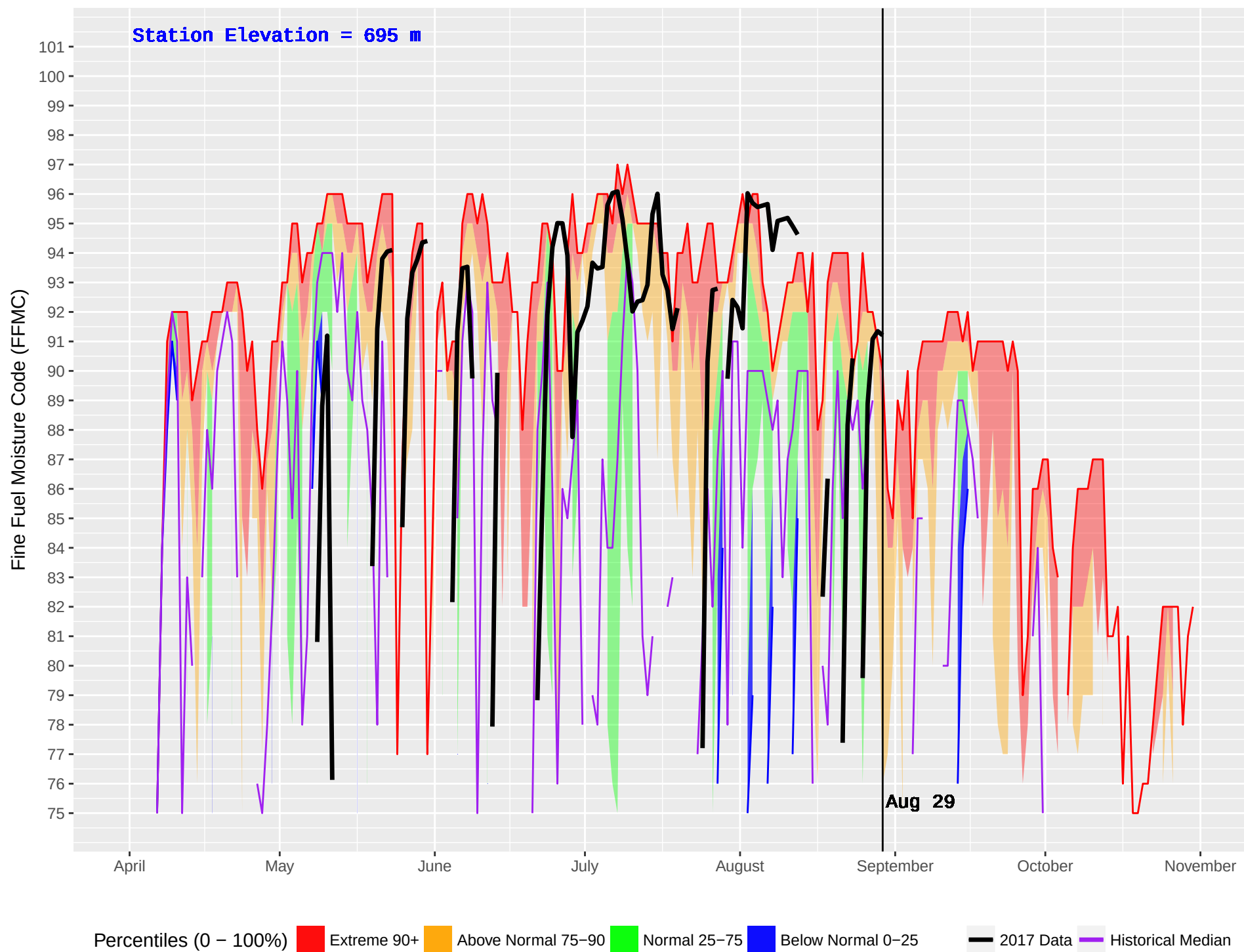
BLUE RIVER 2 (1108) : Historical (2011–2016) and Current (2017) Noon Fine Fuel Moisture Code (FFMC)
