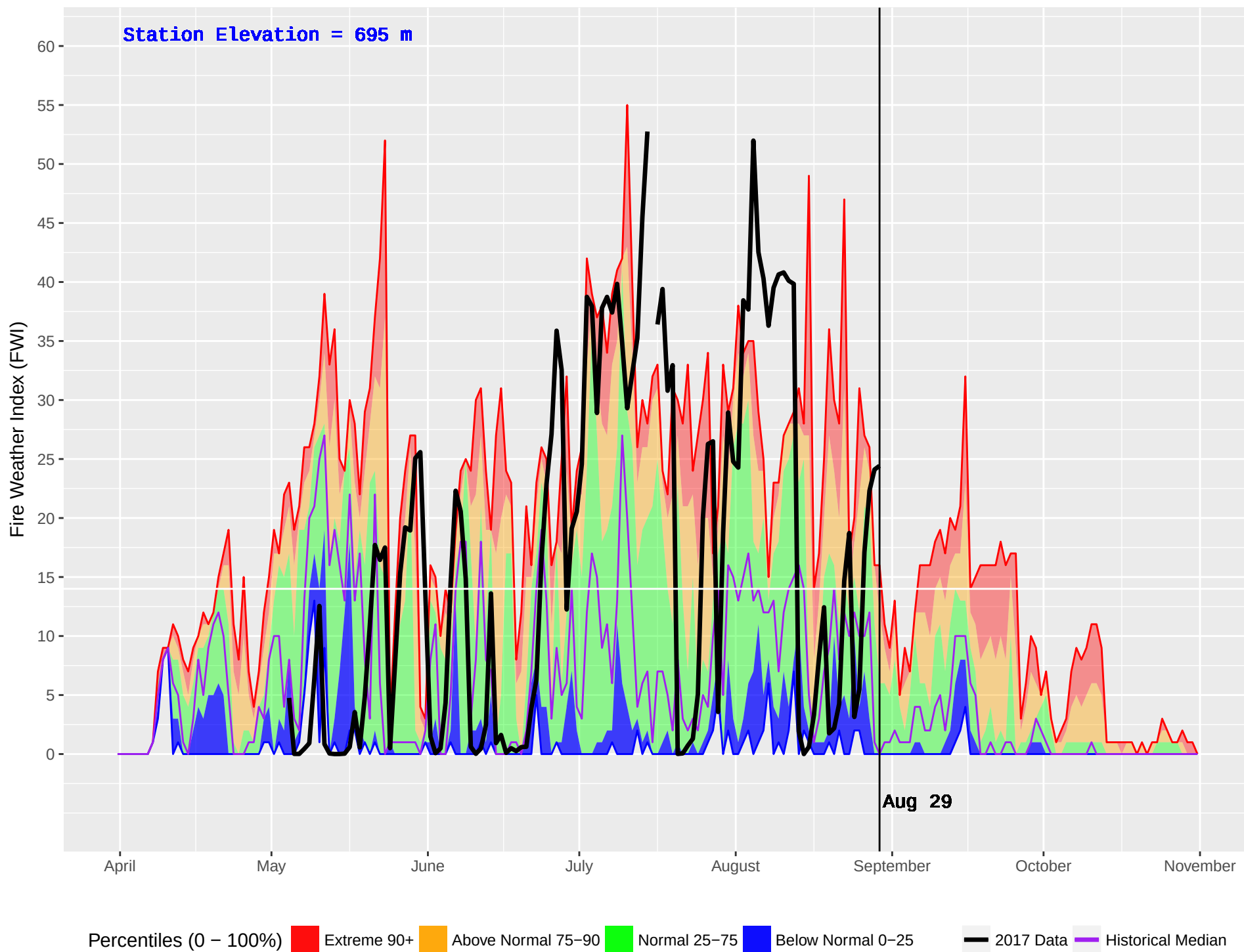
BLUE RIVER 2 (1108) : Historical (2011–2016) and Current (2017) Noon Fire Weather Index (FWI)
