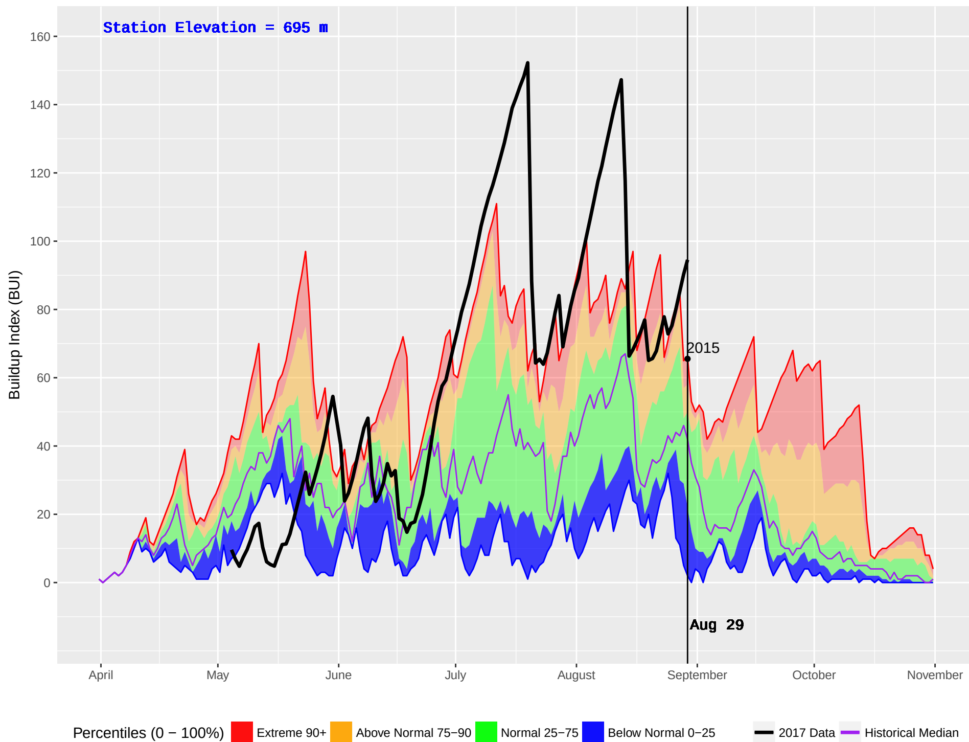
BLUE RIVER 2 (1108) : Historical (2011–2016) and Current (2017) Noon Buildup Index (BUI)
