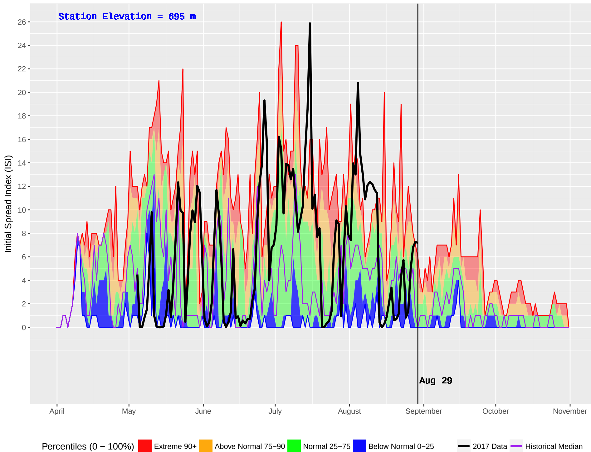
BLUE RIVER 2 (1108) : Historical (2011–2016) and Current (2017) Noon Initial Spread Index (ISI)
