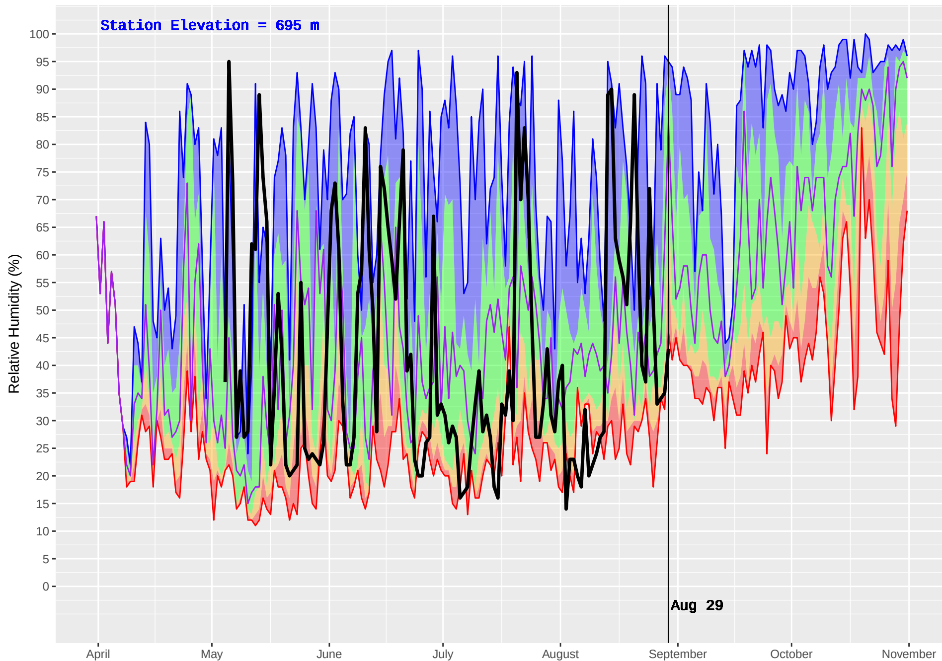
BLUE RIVER 2 (1108) : Historical (2011–2016) and Current (2017) Noon Relative Humidity
