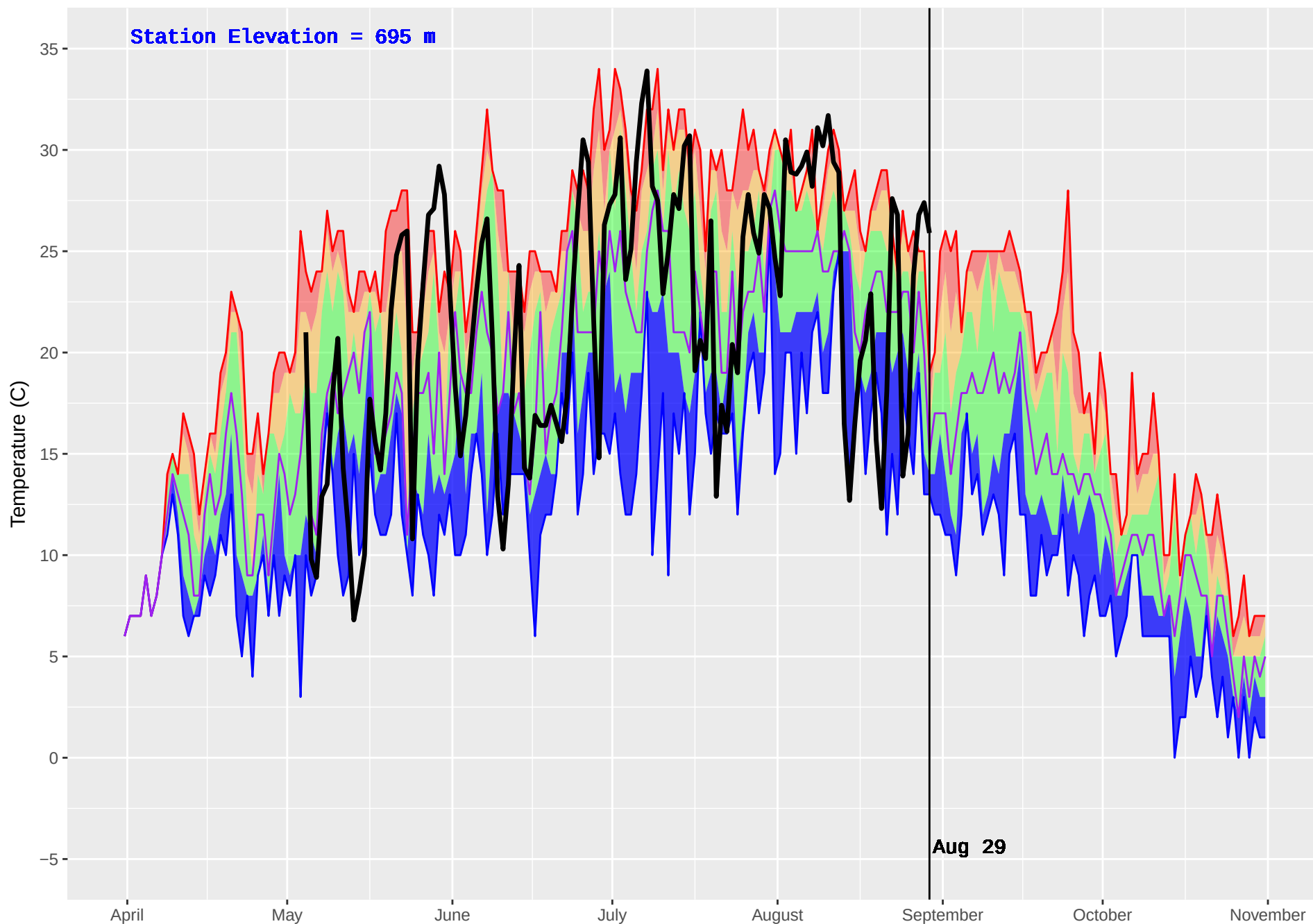
BLUE RIVER 2 (1108) : Historical (2011–2016) and Current (2017) Noon Temperature
