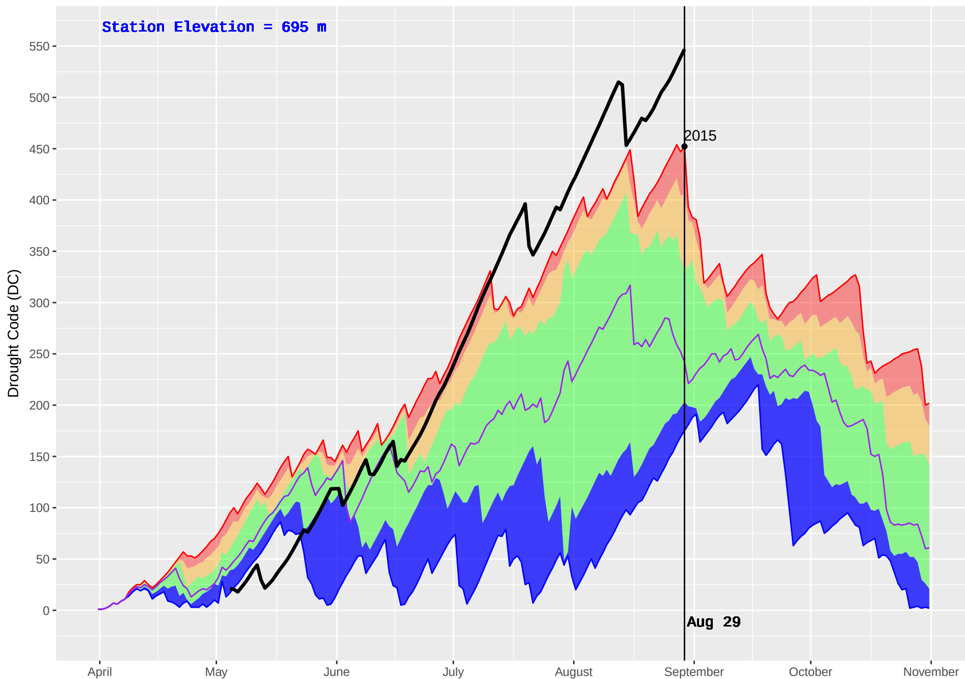
BLUE RIVER 2 (1108) : Historical (2011–2016) and Current (2017) Noon Drought Code (DC)
