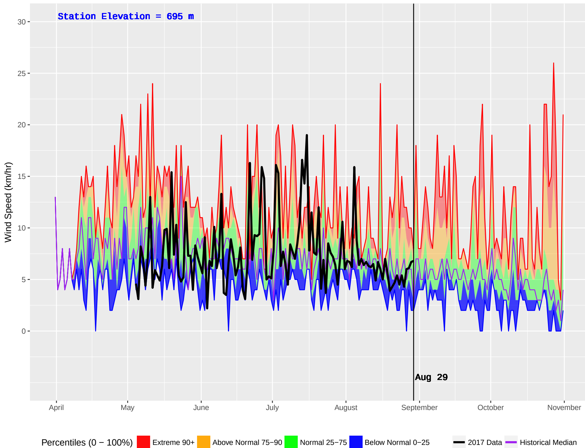
BLUE RIVER 2 (1108) : Historical (2011–2016) and Current (2017) Noon Wind Speed
